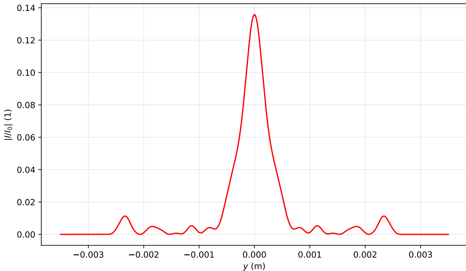
Intensity profile I(x=0, y, z=3.344)/I_0 , P_{in}=9.0P_{cr} , artificial time
